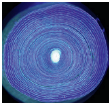
The annual growth rings of a deep-sea coral under ultraviolet light.
