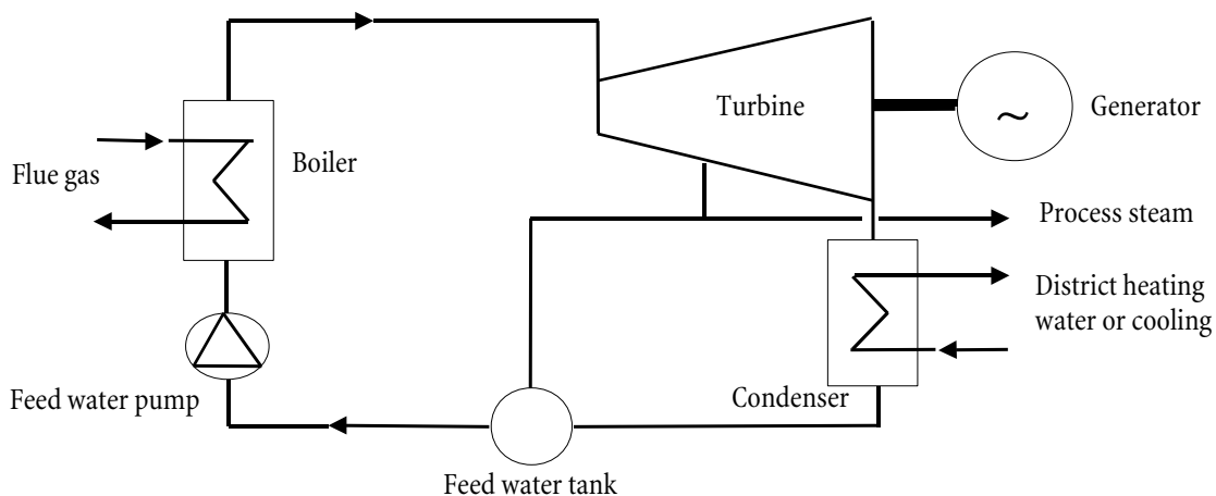
Figure 3.2 The Rankine process
