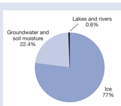
Fig. 1: Distribution of global fresh water. Water vapor in the atmosphere, which accounts for only 0.04% of the total, is not included.
