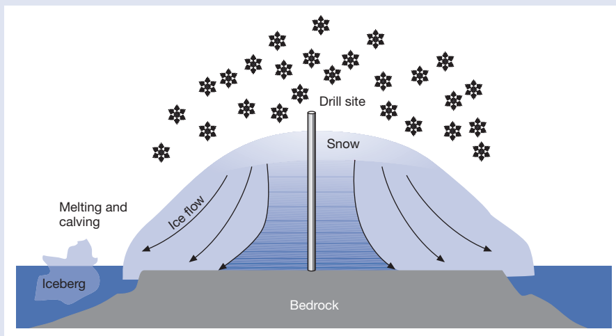
Fig. 3: Cross-section of the polar ice sheet. In the higher parts of the ice sheet, ice is being continually formed from snow. This ice flows slowly towards the coast, where it melts or floats off into the sea as icebergs (a process known as "calving"). This flow of ice means that the annual ice layers become thinner with increasing depth.
