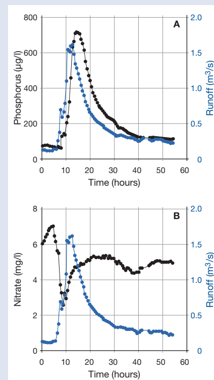
Fig. 2: Concentration dynamics of (A) phosphorus and (B) nitrate (black curves) and runoff (blue curves) during a rain event in a small agricultural catchment area (Kleine Aa at Lake Sempach in the canton of Lucerne) [3]. Pesticides, heavy metals and sediments usually show dynamics similar to phosphorus.
