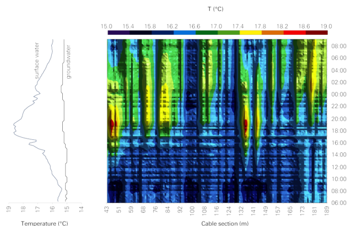
Fig. 3: Temperatures measured in the Chriesbach (Canton Zurich) in summer 2014, from 06:00 to 09:00 on the following day. The curves on the left indicate surface water (light blue) and groundwater (black) temperatures. The colour plot on the right shows streambed temperatures measured along a roughly 150-metre section of buried fibre-optic cable. It is apparent that in certain zones virtually no warm surface water flows past the cable into the groundwater (e.g. the section from 95 to 105 metres), while in others (e.g. at 47 and 137 metres) daily variation in surface water temperatures is clearly reflected in the streambed.
