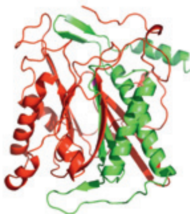
The three-dimensional structure of the BapA enzyme helps to explain the mechanisms of its catalytic action. X-ray analysis of the crystallized enzyme was performed at the PSI in collaboration with Professor Markus Grütter of Zurich University.
