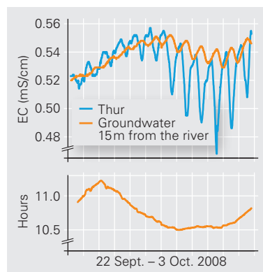
The diurnal variation of electrical conductivity (EC) in the Thur and in an adjacent groundwater well (top) can be used to calculate the travel time of infiltrating river water (bottom).
