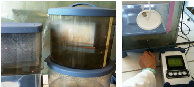
Figure 14 PreSens oxygen spots (red dots) placed in the filters (photo M. Peter and A. Florin)
