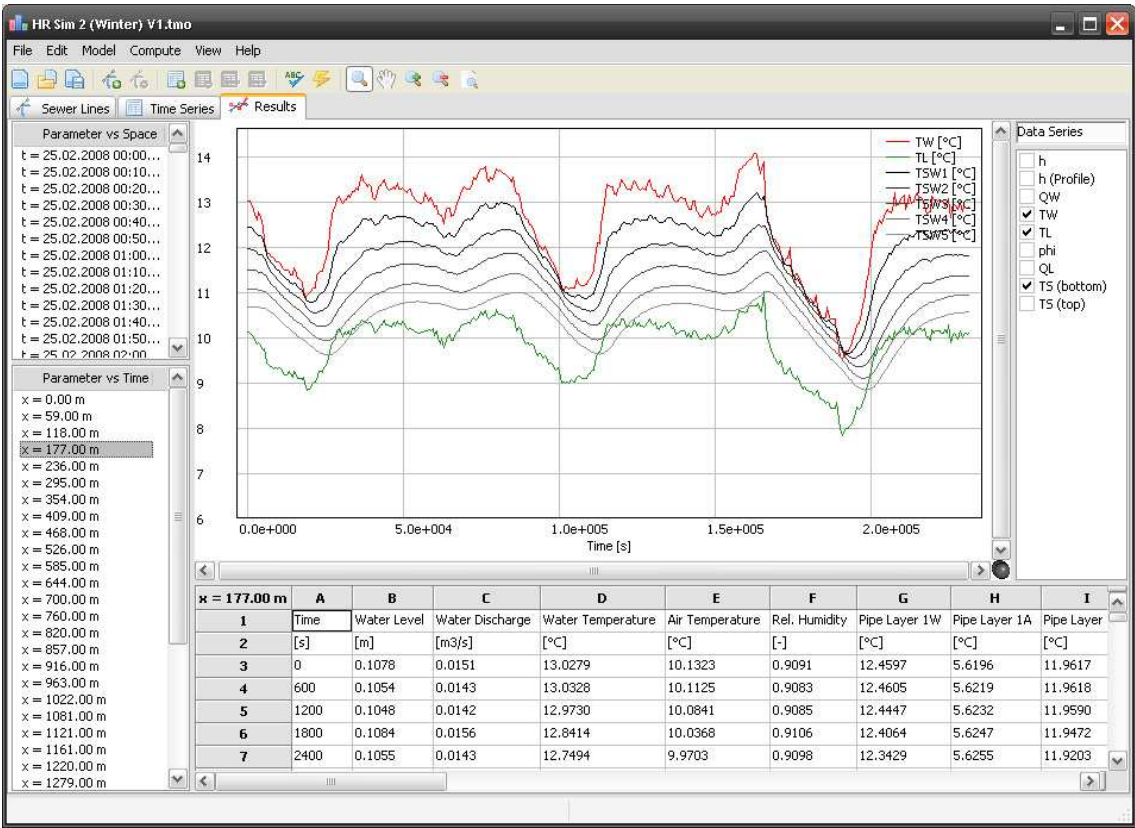
Figure 2.17.: Main window displaying the calculation Results tab. The wastewater and sewer air temperature as well as the temperature of the pipe layers are plotted.
