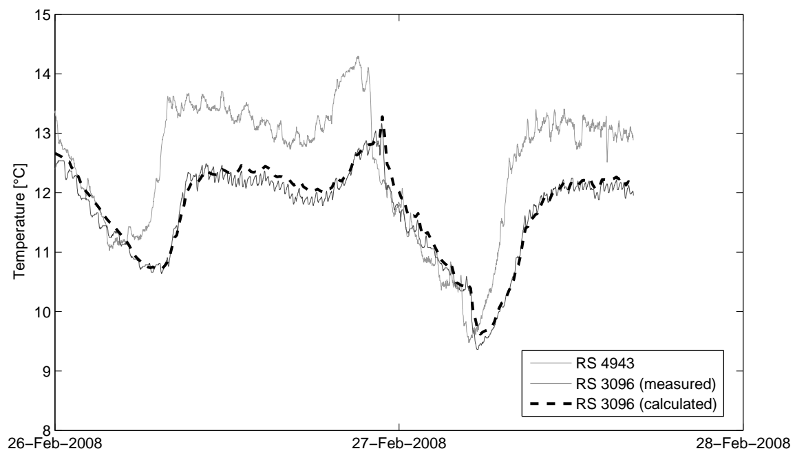
Figure 3.9.: Result of the model calibration.
