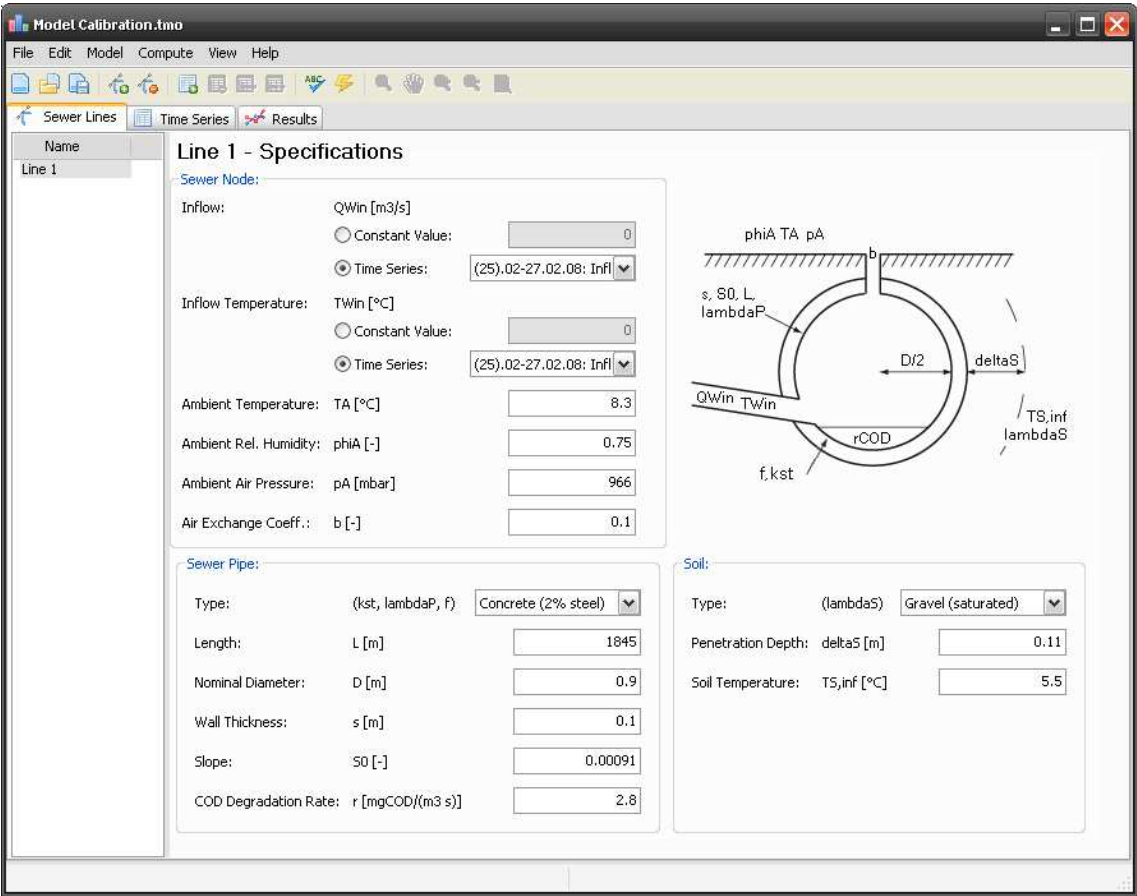
Figure 3.4.: The Sewer Lines tab. A new, empty sewer line has been added to the model and the parameter values of Table 3.1 have been entered.
