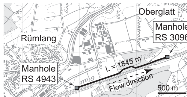
Figure 3.1.: Top view of a section of the sewer between the villages Rümlang and Oberglatt in the Canton of Zurich, Switzerland
