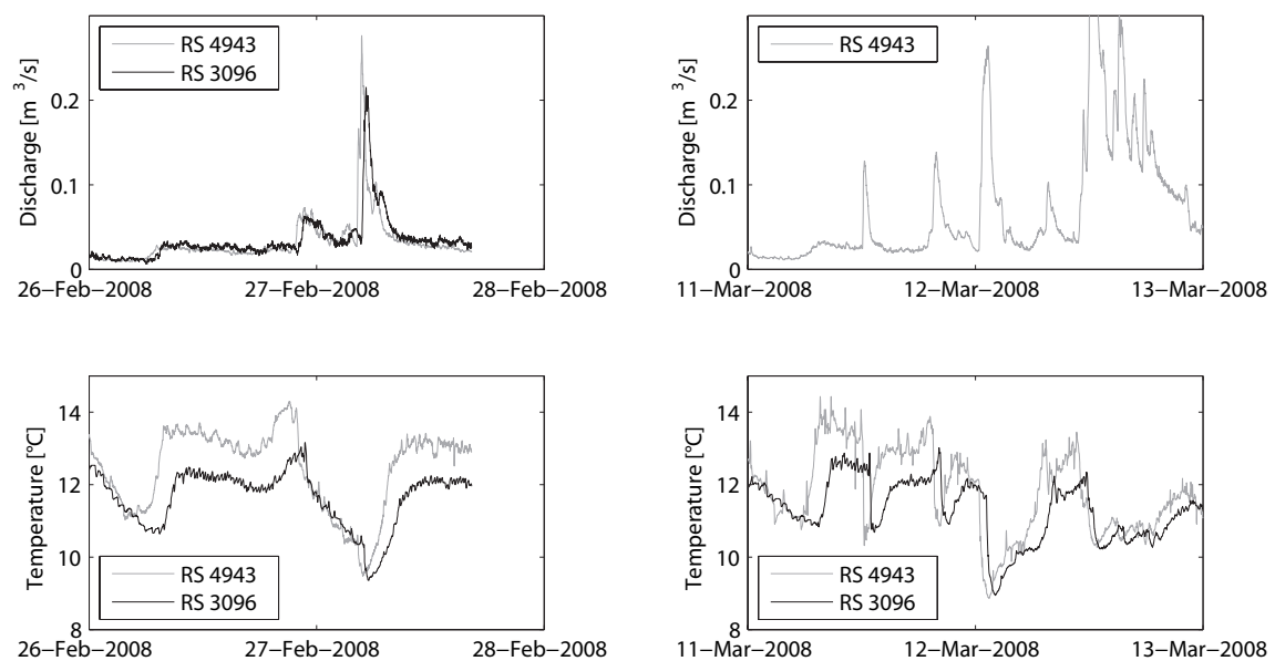
Figure 3.2.: Discharge and temperature data measured from February 26 to February 28 (left column) and from March 11 to March 13 (right column) at the manholes RS 4943 and RS 3096.
