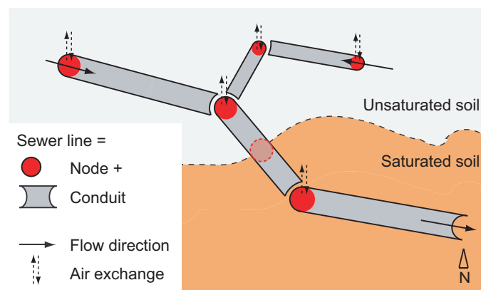
Figure 2.2.: Discontinuities require that nodes are introduced, which separate sewer conduits having different properties.
