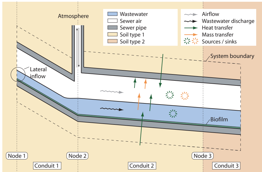
Figure 2.3.: Compartments and processes considered in the sewer model. Complex systems can be modeled by series of the elements "node plus conduit".
