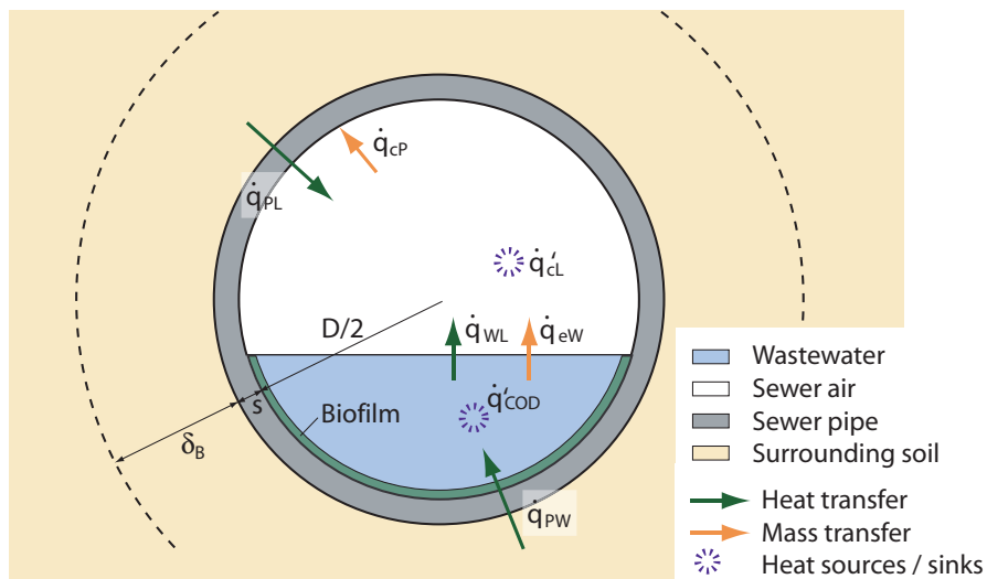
Figure A.1.: Cross-section of a sewer line with transfer processes by which the humidity in the sewer headspace and the temperatures in the wastewater, sewer headspace, sewer pipe and soil are affected.
