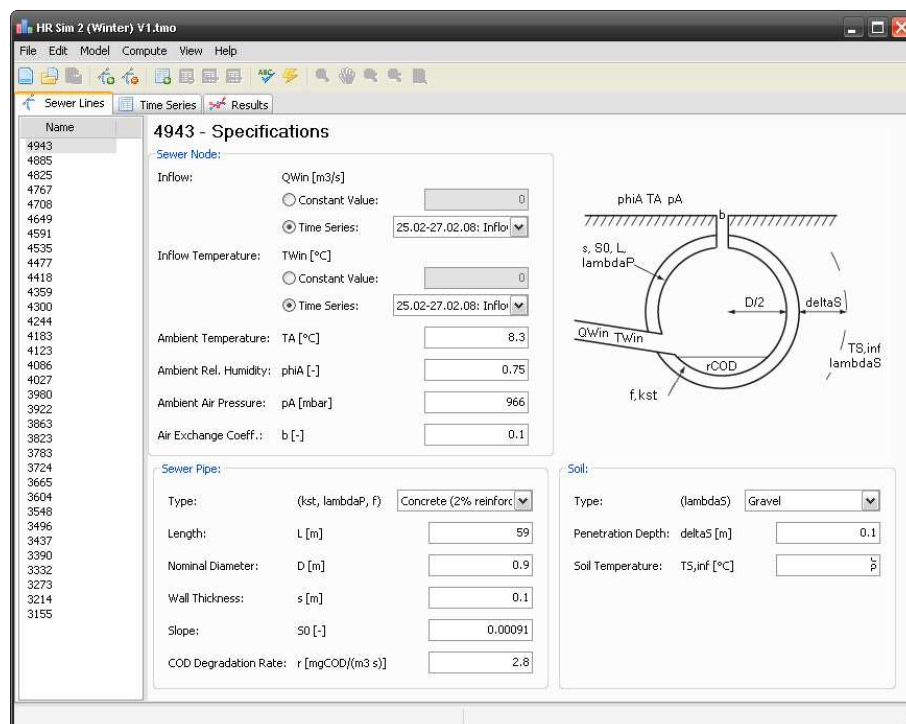
Figure 2.5.: Main window displaying the Sewer Lines tab completed with values.
