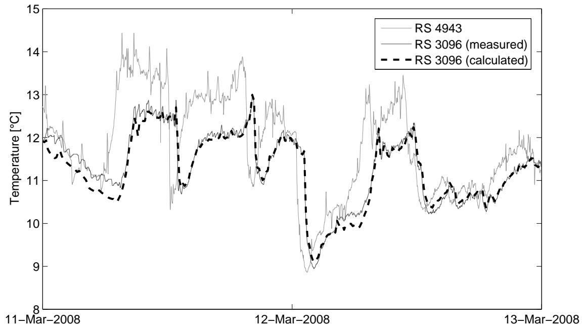
Figure 3.10.: Result of the model validation.
