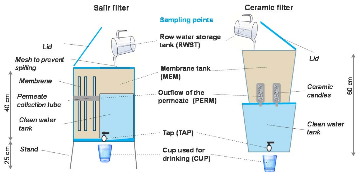
Figure 25 Drawing of the Safir and ceramic candle filters with major sampling points (Derksen S., and Graf V., 2013)
