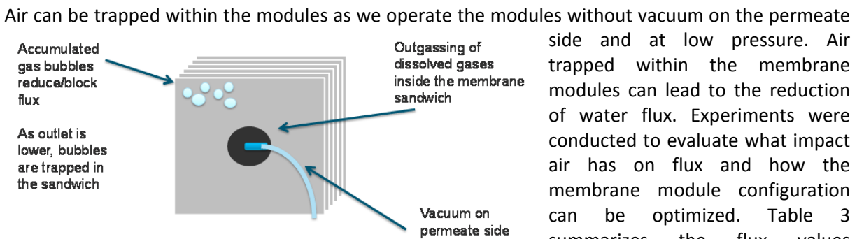
Figure 5 Schematic presentation of the air trapping within the Microdyn module (by S.Derksen)
