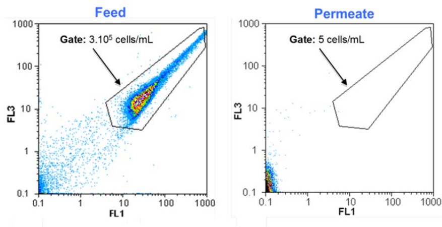
Figure 31 Flow cytometry dot plots of the feed spiked with fluorescently labeled B. diminuta , and the permeate (Peter-Varbanets, et al., 2010)
