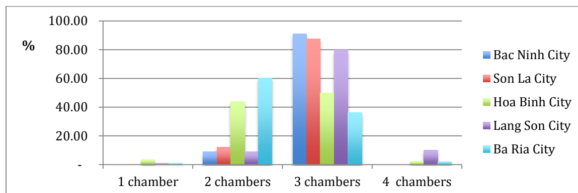
Figure 5: Septic tanks' chambers in 5 cities
