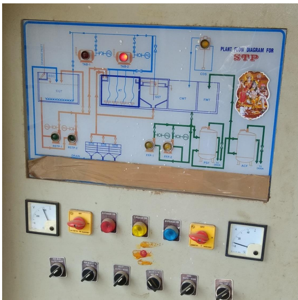
Figure 14: SSTS control panel with flow diagram (Photo: Sunil Kumar).
