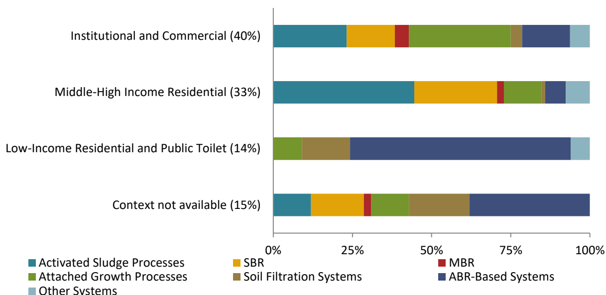
Figure 16: Distribution of treatment technologies in different contexts of application (n=279).
