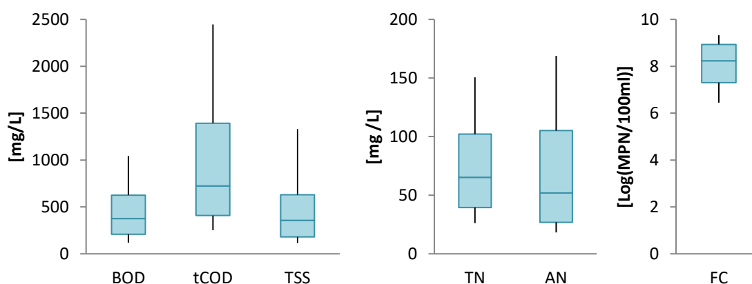
Figure 37: Box plots (0.1, 0.25, 0.5, 0.75 and 0.9 percentiles) of inflow wastewater characteristics from 40 sampled SSS systems (three rounds of 24 h composite sampling).
