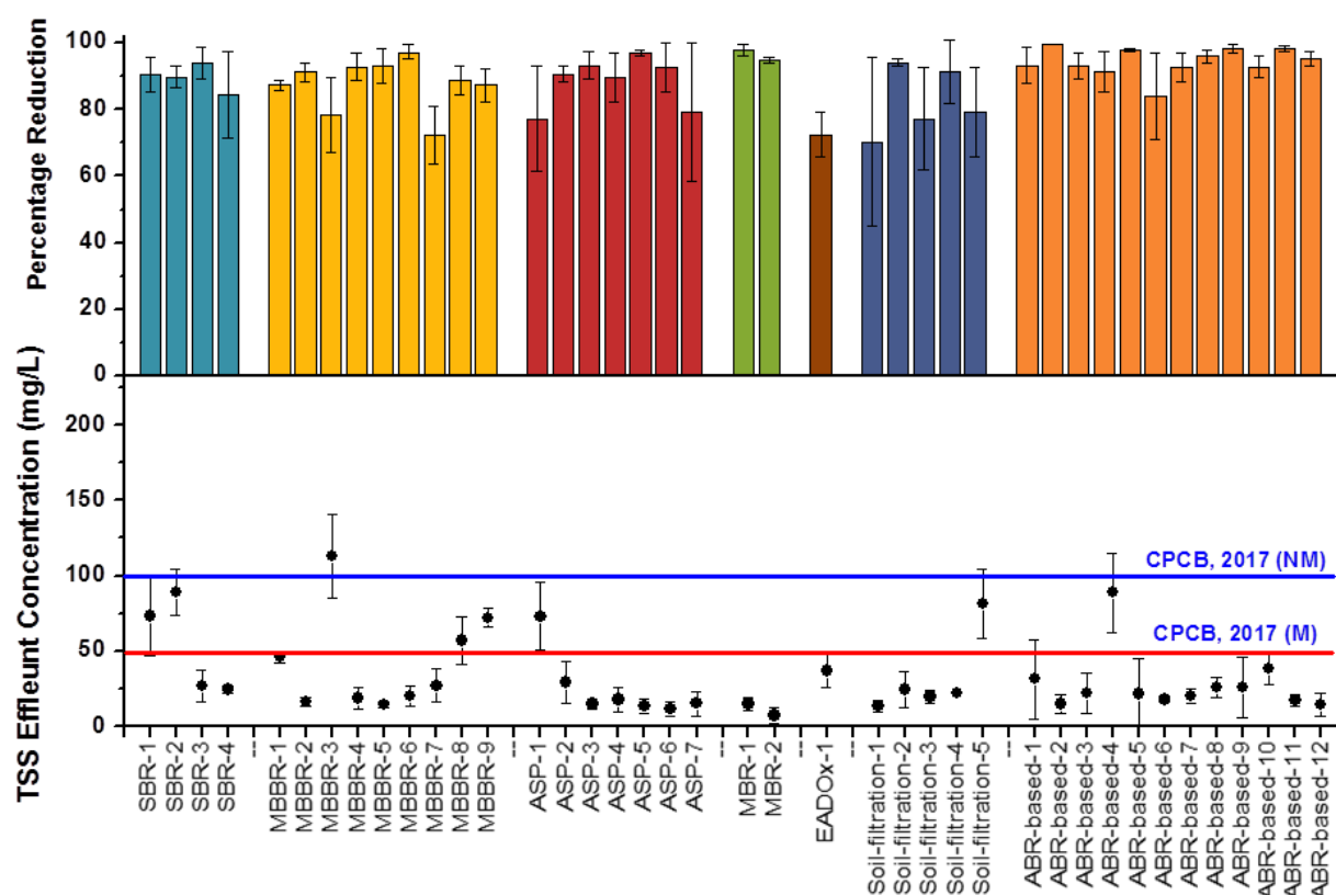
Figure 43: Average (three rounds of 24 h composite sampling \pm std. dev.) TSS removal efficiency and treated water quality (M: Metro; NM: Non-Metro).
