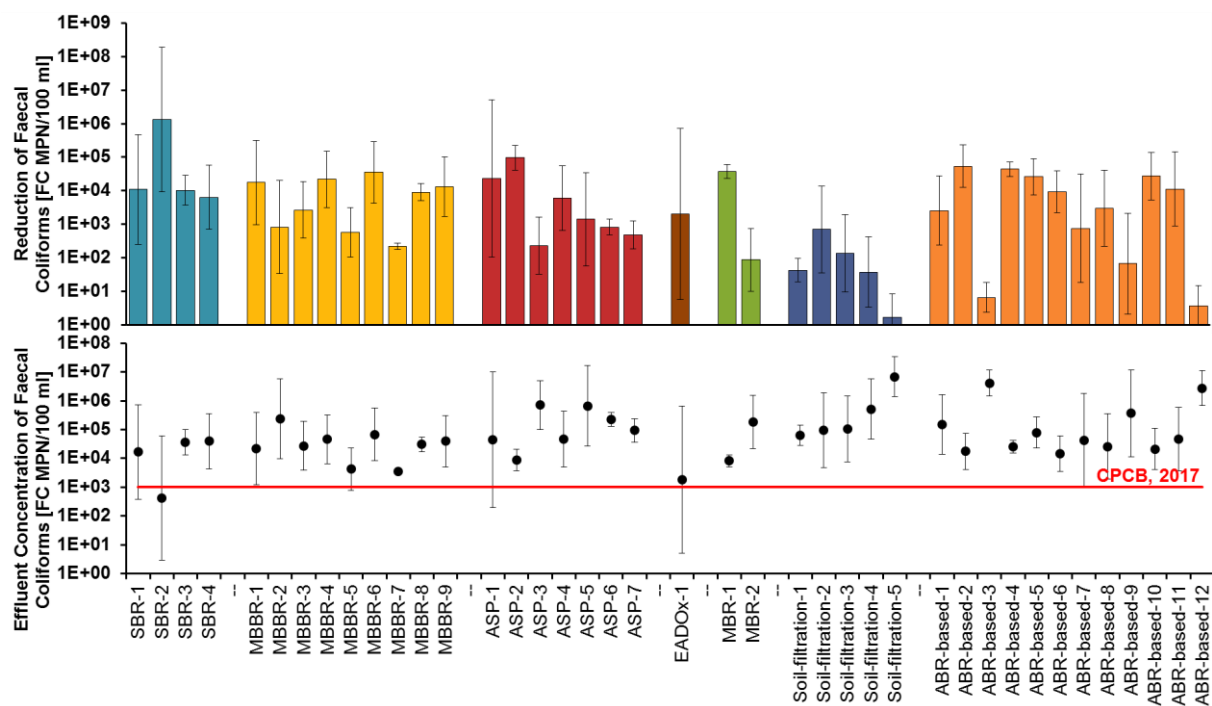
Figure 47: Average (three rounds of 24 h composite sampling \pm std. dev.) faecal coliforms concentration reduction and treated water quality.
