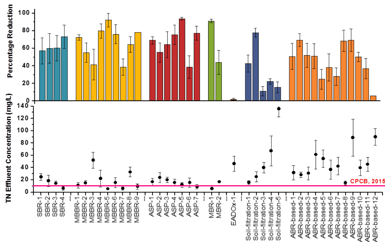
Figure 45: Average (three rounds of 24 h composite sampling \pm std. dev.) total nitrogen removal efficiency and treated water quality.
