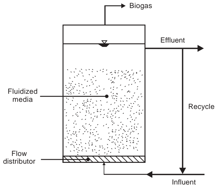
Figure 19: Fluidized Aerated Bed (FAB) Reactor
