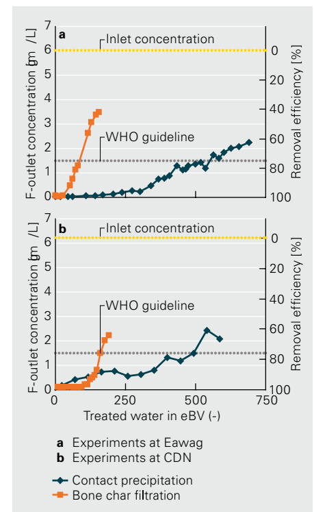
Figure 1: Fluoride breakthrough curves as a function of treated water in empty bedvolumes (eBV).
