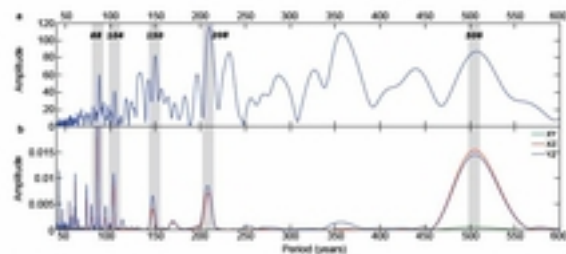
Fig. 1. Comparison between solar activity and planetary torque in the frequency domain. (a) Fourier spectrum of the solar activity quantified by the solar modulation potential. (b) Fourier spectrum of the annually averaged torque modulus. Both these correspond to case 1, and to case 2, and given in case 3. The spectra display significant peaks with very similar periodicities. The 11 yr (Schwabe) and the 22 yr de Vries cycles are the most prominent, but periodicities around 104 yr, 130 yr, and 104 yr are also seen.
